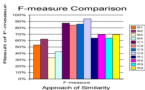
Gambar 3 Perbandingan F-measure
