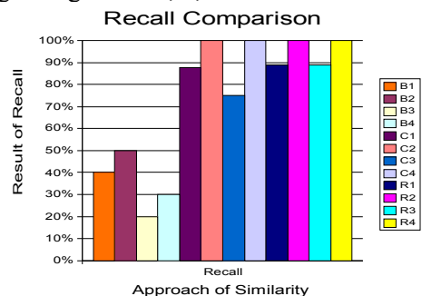
Gambar 1 Perbandingan Recall
